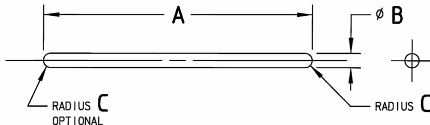
FIGURE 1 - WIRE, RETAINER
